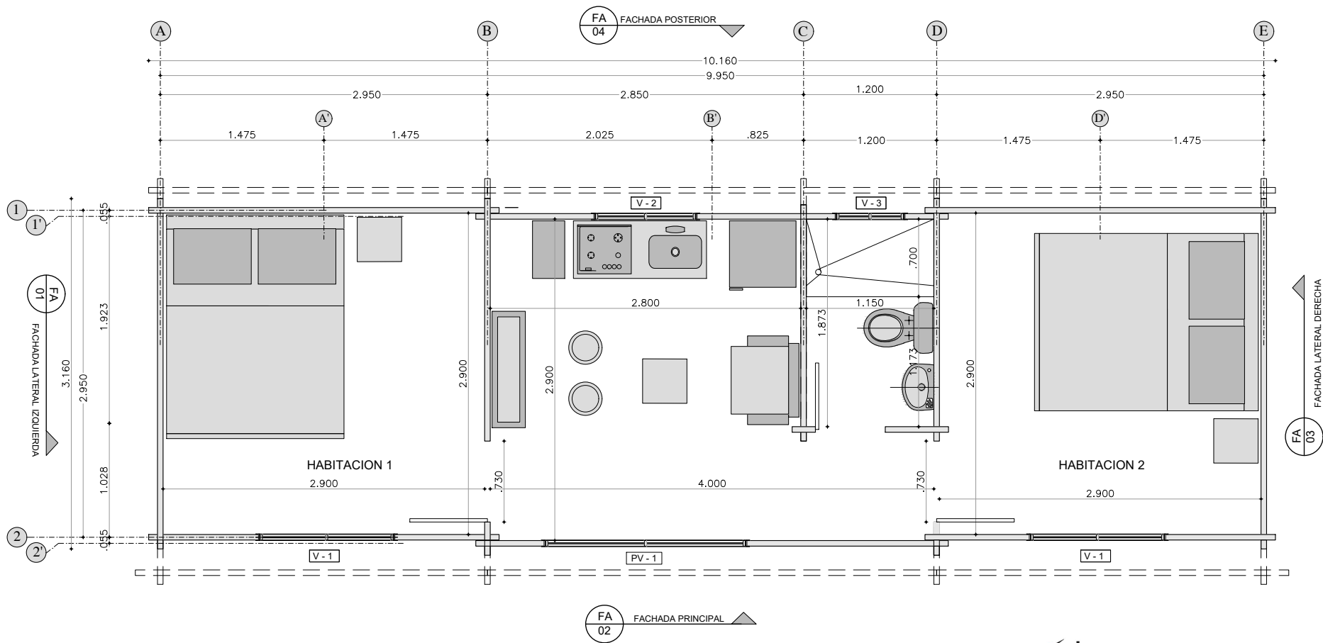
PLANTA GENERAL TINY HOUSE 30 M2
